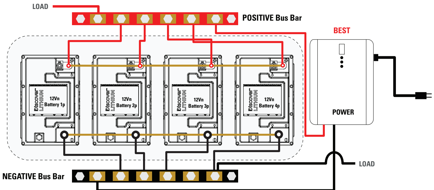
Figure 7: Parallel connection 4P x 12Vn = 12V
