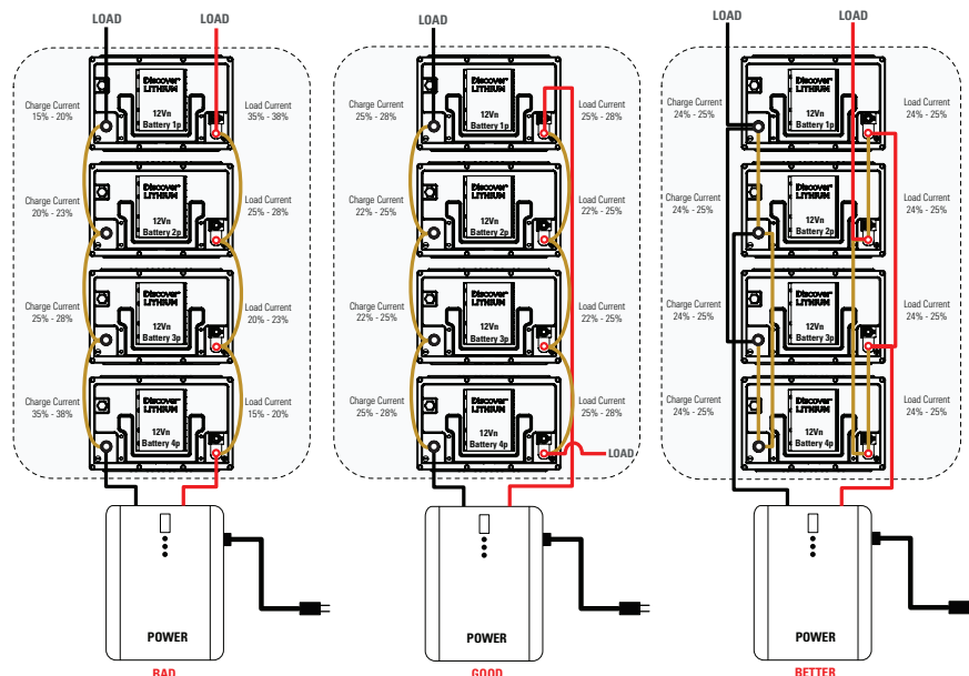
Figure 6: Cabling options for charging batteries in parallel
