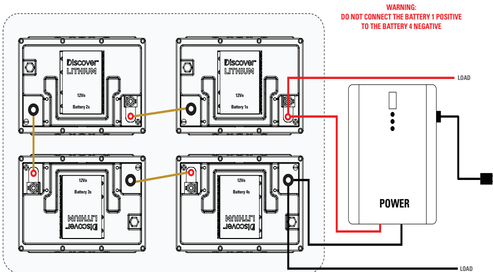
Figure 2: Series Connection 4 x 12.8Vn. BMS will protect at 58.4V
