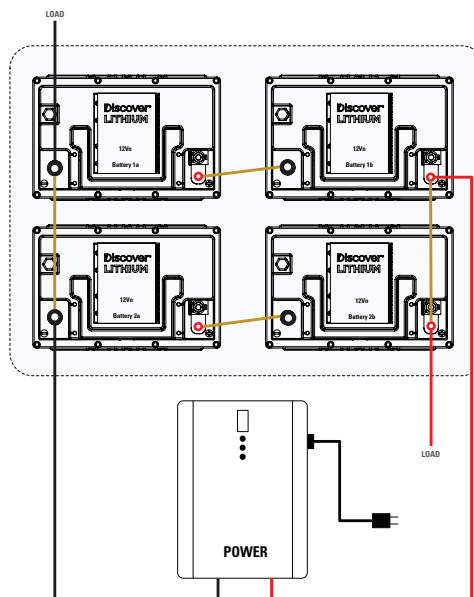
Figure 8: Series and parallel bank using 2 strings of 2 x 12V batteries in series then paralleled
