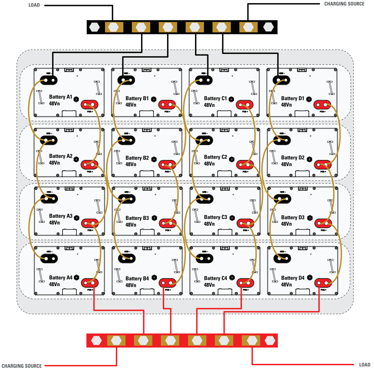
Figure 5: Illustrates 4 strings of 48V nominal 30AH lithium batteries connected in parallel and then paralleled onto negative and positive BUS bars creating a 48V 480AH battery bank
