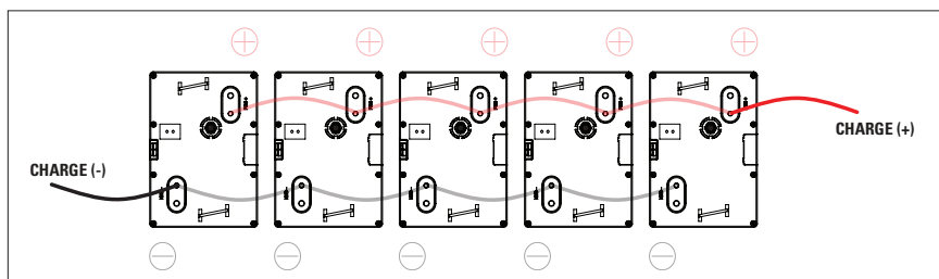
Figure 8. Branchements de charge
