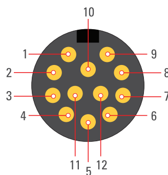
Circular 12 PIN
