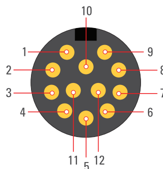
Circular 12 PIN
