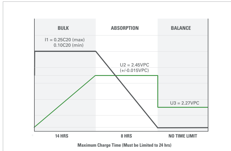
Figure 1: Voltage Regulated Charge profile (IUU charger) at 25°C (77°F)
